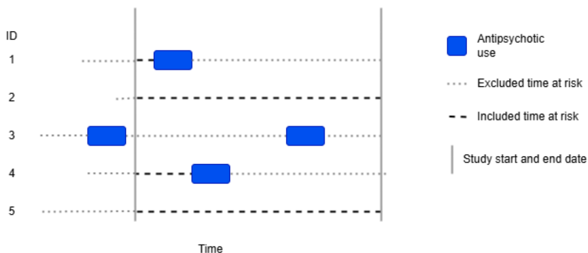
Figure 4. Illustration of incidence calculations.
