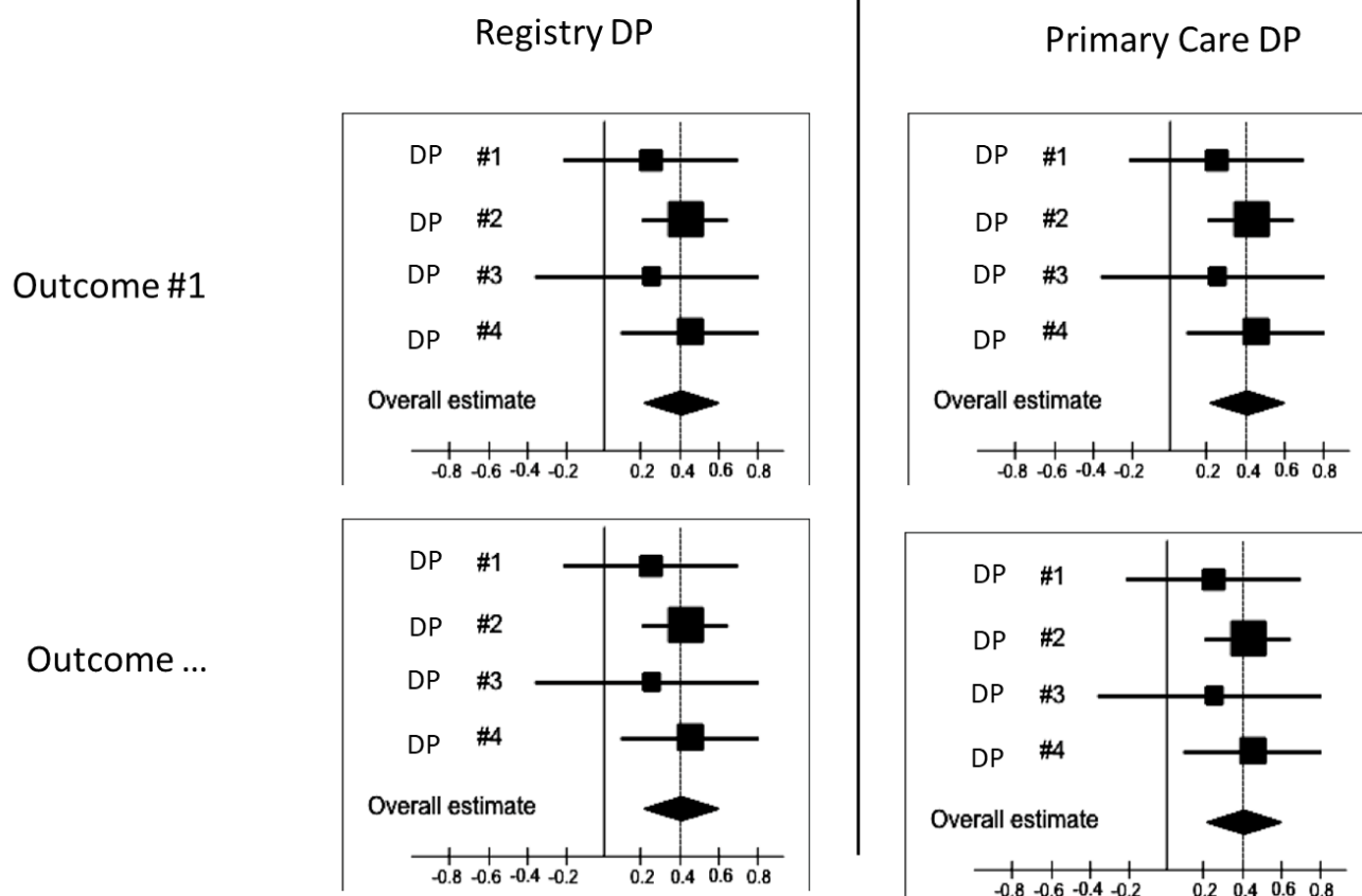
Figure 6. Example of pooled incidence rates of AESI in registry and primary care only data sources.
