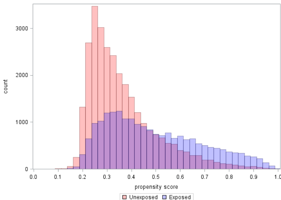
Figure 1 Distribution of PS for vaccinated and unvaccinated subjects in a random sample of the study population
