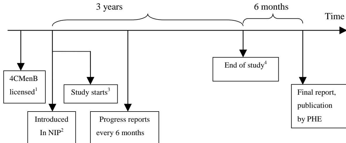
Figure 4 Study Timelines
