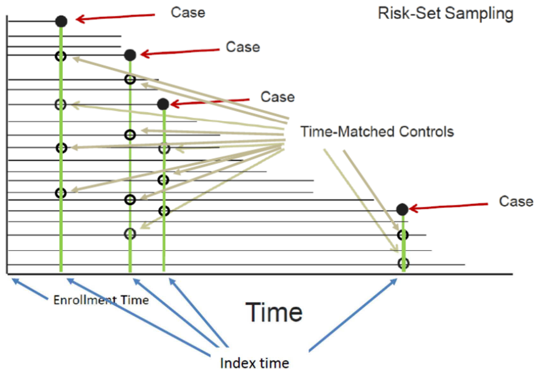
Figure 2. Matching Using Incidence-density Sampling
